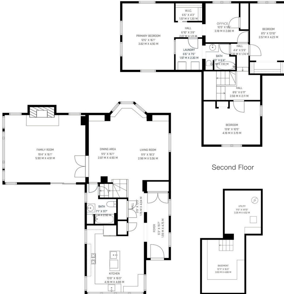
Ground Floor
